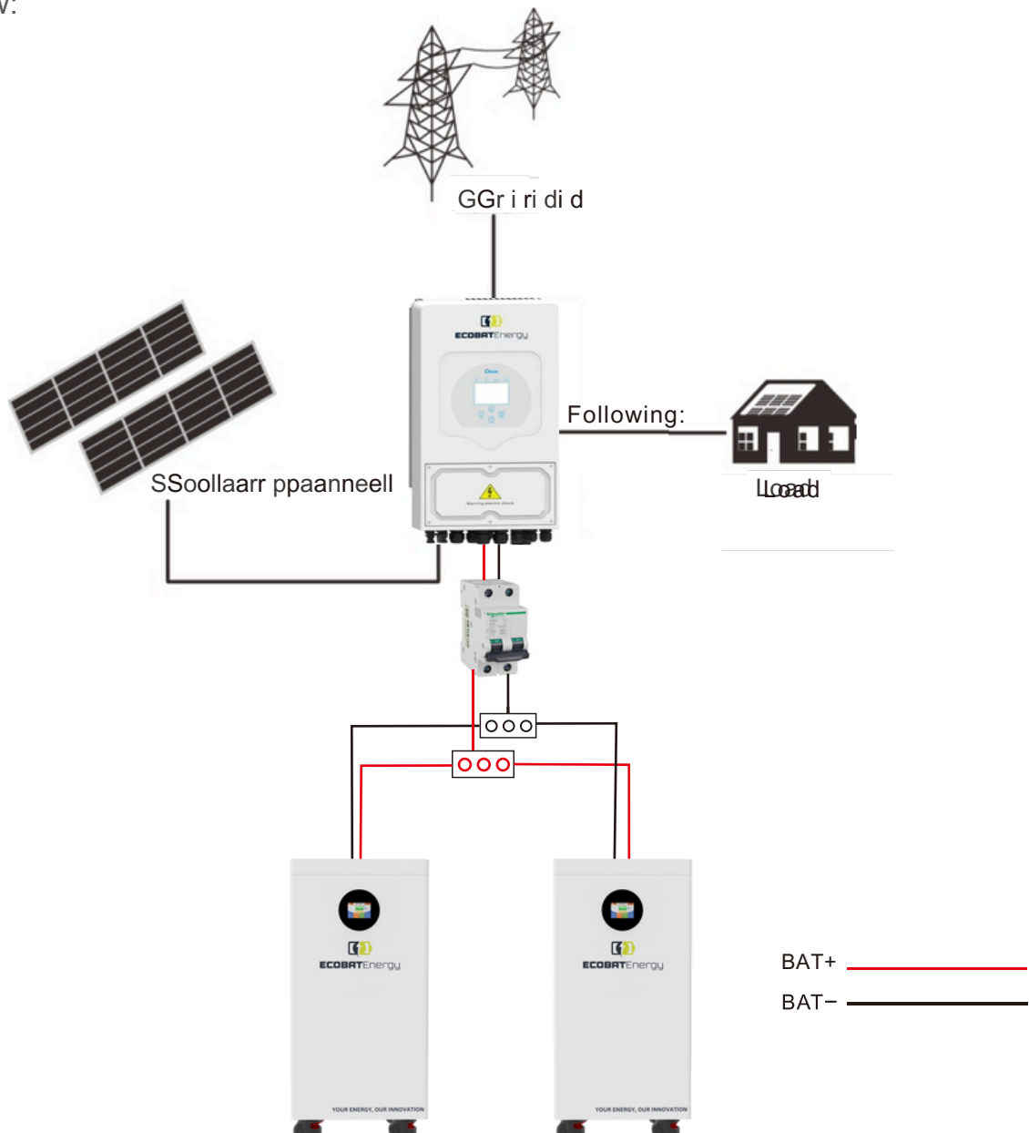
Figure 1 Operation Principle Diagram of Battery System
